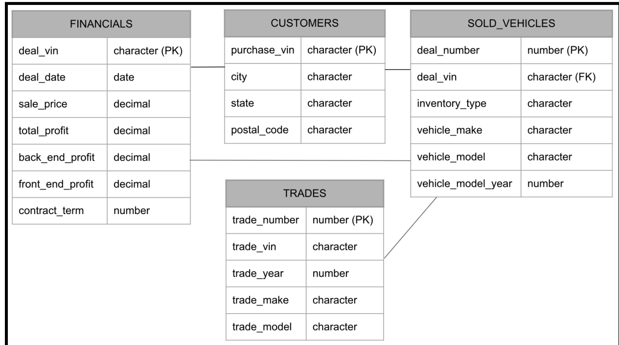
Diagram 1: Luxury_Car_Dlrshp ERD
